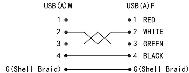
WIRING DIAGRAM
