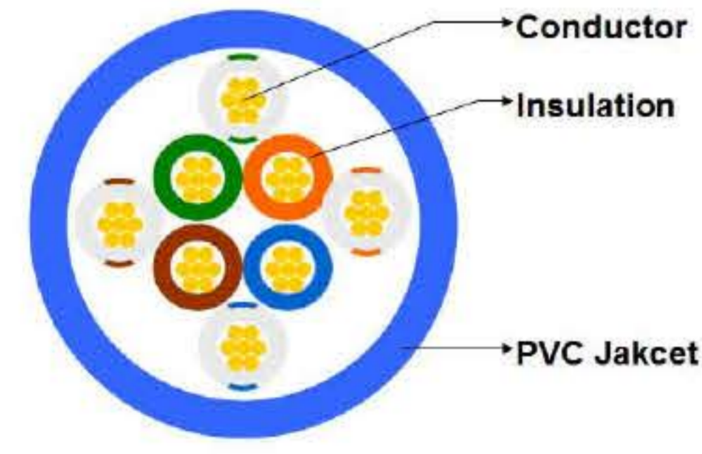
CABLE CROSS-SECTION
