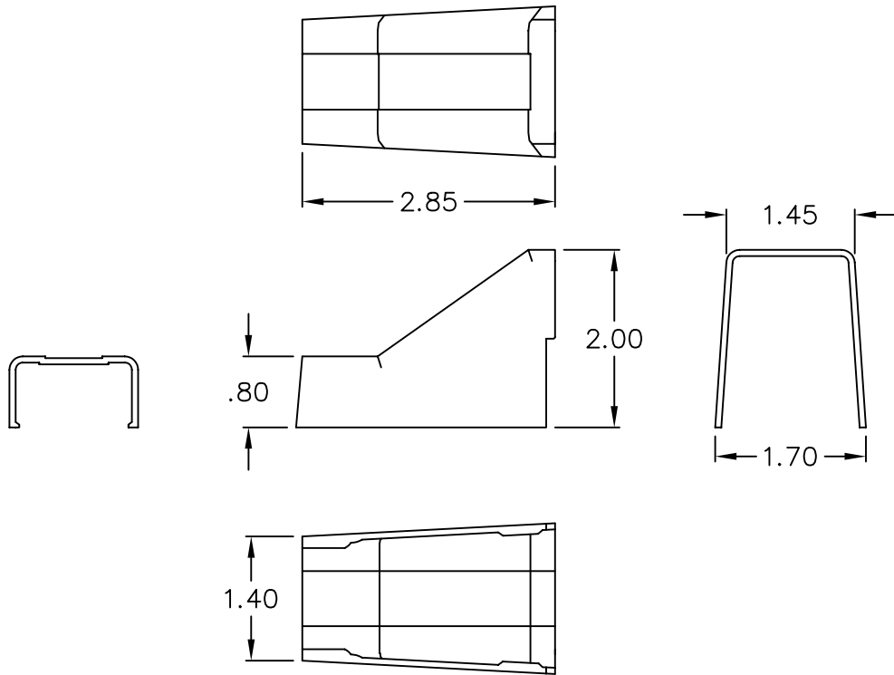
3/4" CEILING ENTRY
